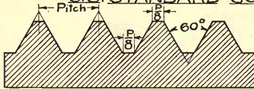
PROFILE OF THREAD
